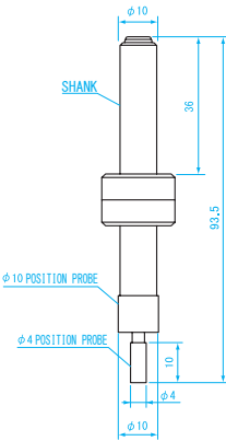
SR-104L (Long probe type)
