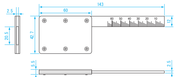
Step measurement between manhole and road surface
