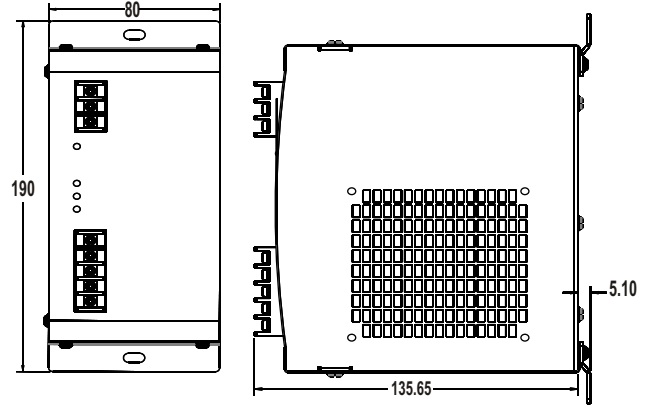
OPS2x3-40
