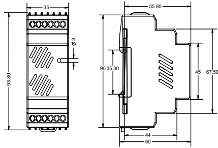
RP-2M-1.1A-24VDC
